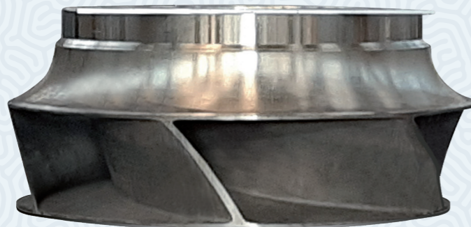
Pump impeller Ø 3000 ◀
